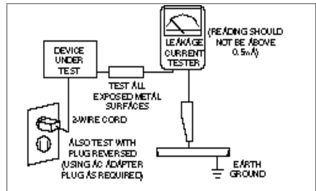
Fig. 1-1 AC Leakage Test
